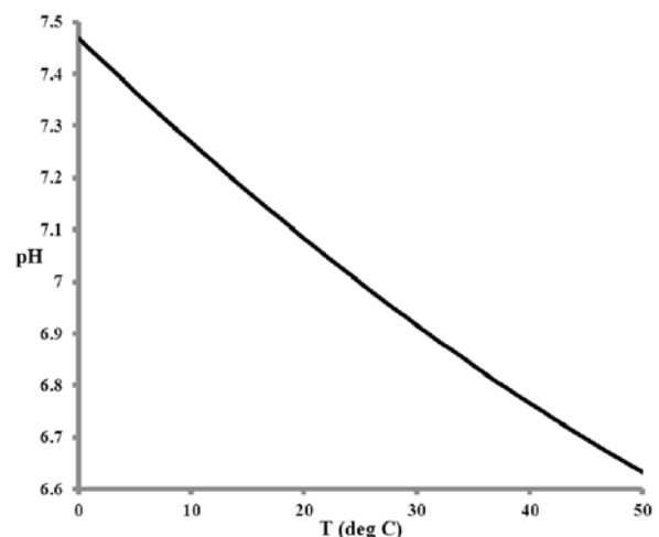
Figure 1. The pH of pure water v temperature*
