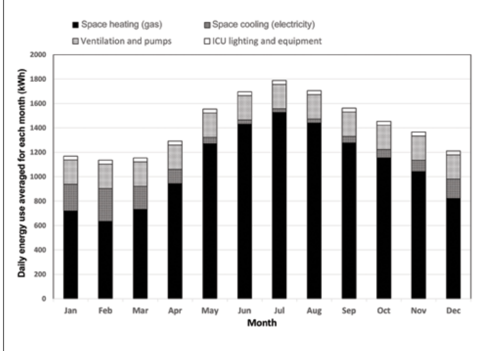
Figure 2. Daily Australian intensive care unit (ICU) gas and electricity use (kWh)
